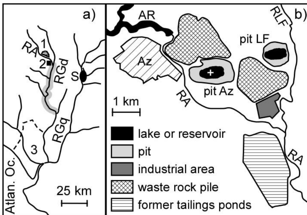
Figure 1. Location of the Aznalcollar pit lake. Panel a): 1 – mining area, 2 – former tailings ponds, 3 – Donana national park, S – Sevillia, RA – Rio Argio, RGd – Rio Guadamar, RGq – Rio Guadalquivir, Atlan. Oc. – Atlantic Ocean, gray area – area contaminated by the failure of the tailings dam in 1998. Panel b): Az – Aznalcollar, RA – Rio Argio, AR – Agrio reservoir, RLF – Rio Los Frailes, pit Az – pit Aznalcollar, pit LF – pit Los Frailes
