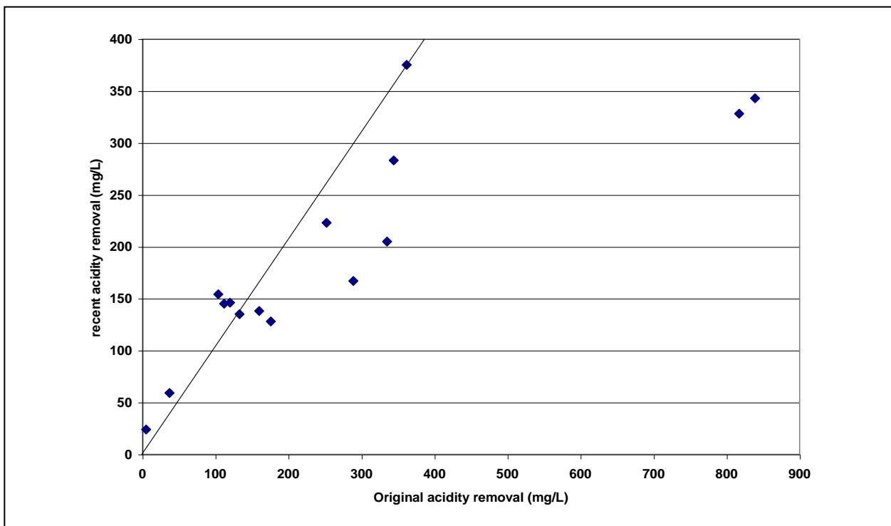
Figure 3. Change in acidity removal from original period to recent period. Line indicates the 1:1 relation expected for no change in removal.
