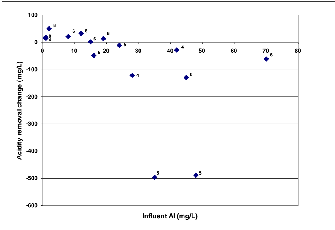
Figure 6. Change in acidity removal (mg/L) as a function of influent Al concentration. Change is from data prior to 2001 vs. more recent data (Table 4). Numbers next to points are the number of years the site has experienced inflow.
