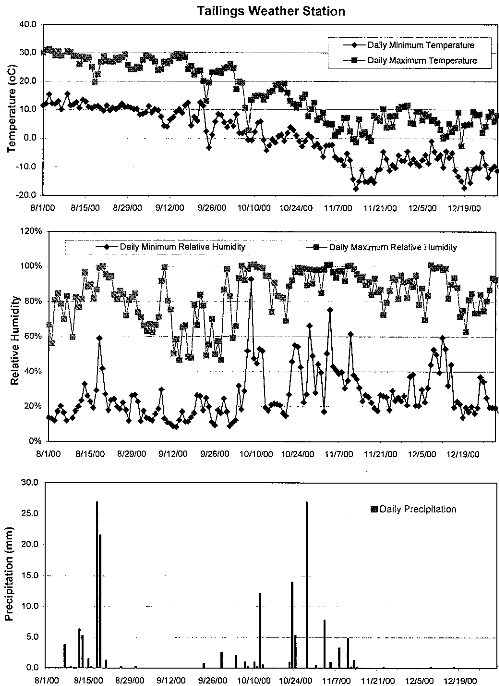
Figure 5. Time trends of temperature and relative humidity (daily MIN/MAX) and precipitation for the five months monitoring period.
