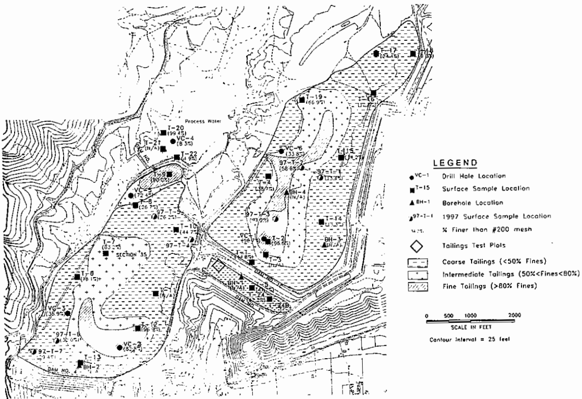
Figure 2. Tailings Characterization Plan for Questa Tailings Facility.
