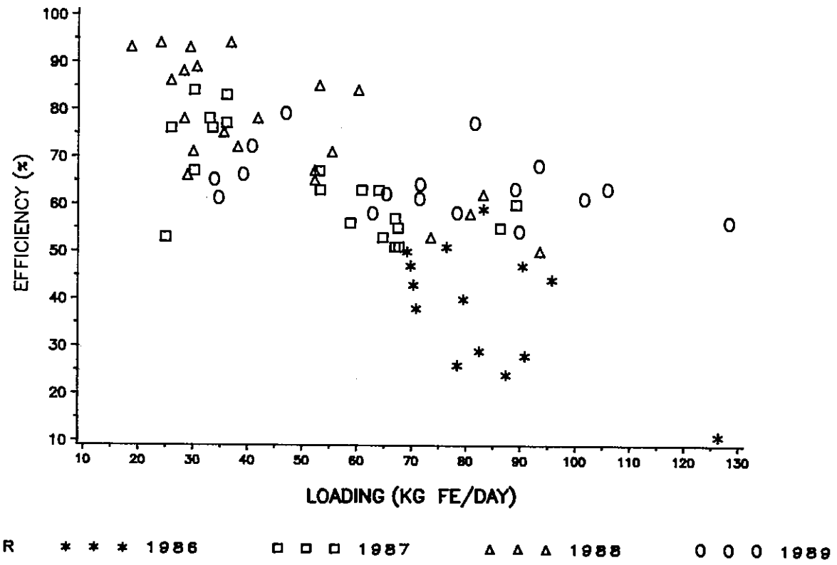
Figure 5. Plot of treatment efficiency for total iron versus iron loading at the Simco wetland (by year).
