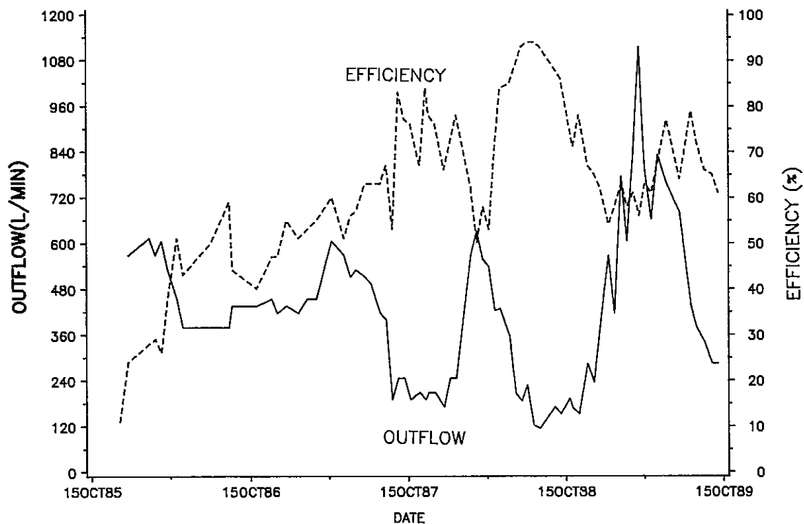
Figure 6. The relationship between treatment efficiency for total iron and outflow at the Simco wetland.
