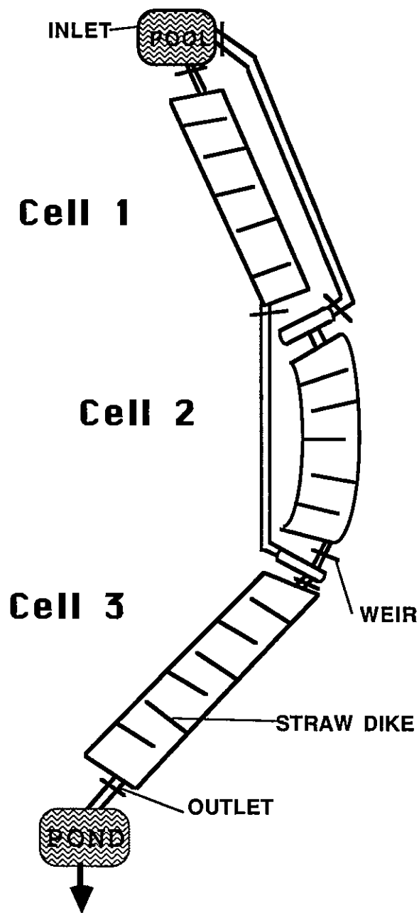
Figure 1. Diagram of the Simco constructed wetland.
