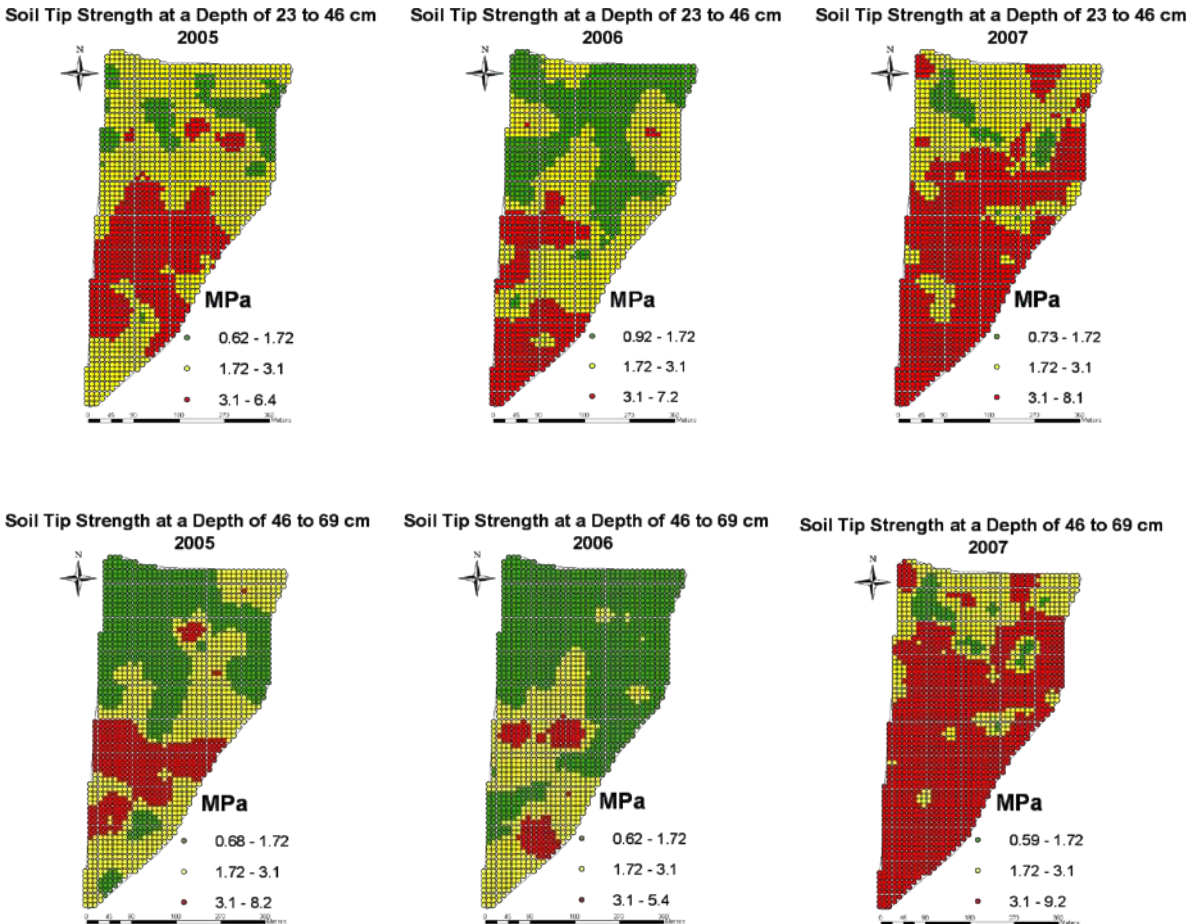
Figure 7. Penetrometer readings (shallow depths) organized by year (going left to right) and depth (going downward). Field areas coded in red signify compacted areas.
