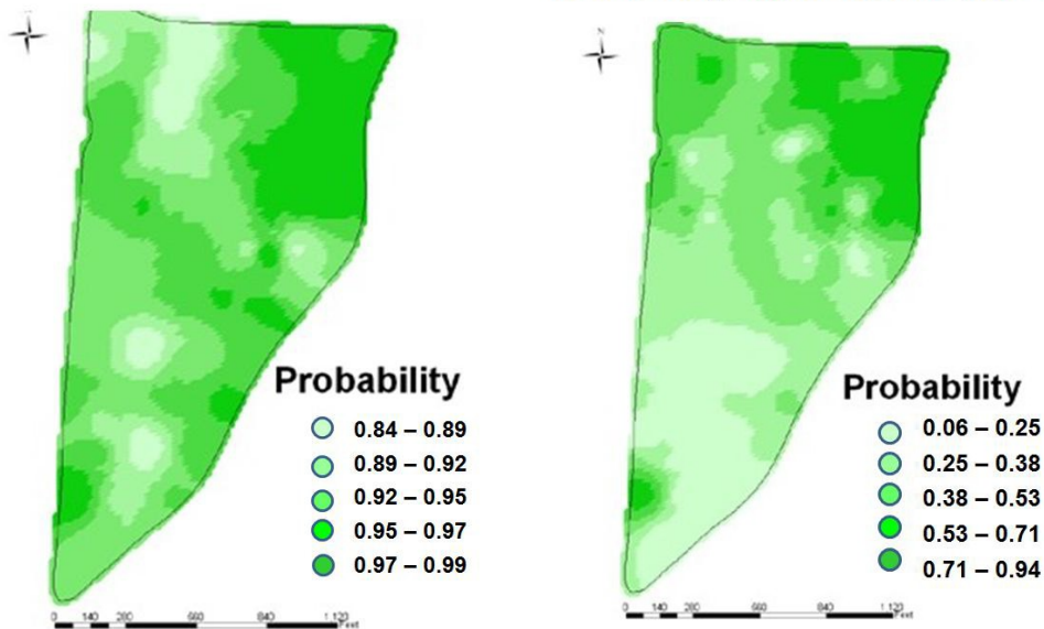
Figure 9. Probability of meeting bond release standards across years for the Lewis field
