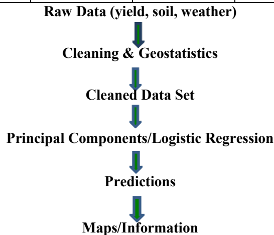
Figure 4. Flow chart of model-building process.
