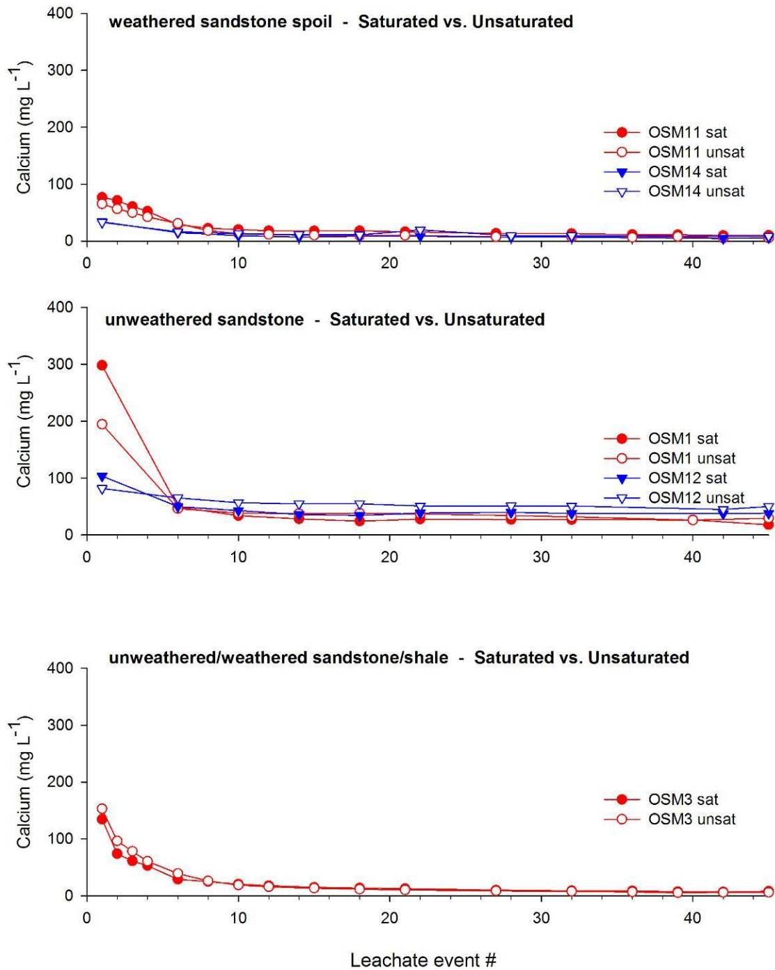
Figure 11. Leachate Ca from weathered and unweathered sandstone spoil under saturated and unsaturated conditions. The 45 leachate events occurred over 22 weeks. Note: for Ca graphs Y-axis ranges from 0 – 400 mg L -1 for Fig. 11, and 0 – 800 mg L -1 for Figs. 12 and 13.
