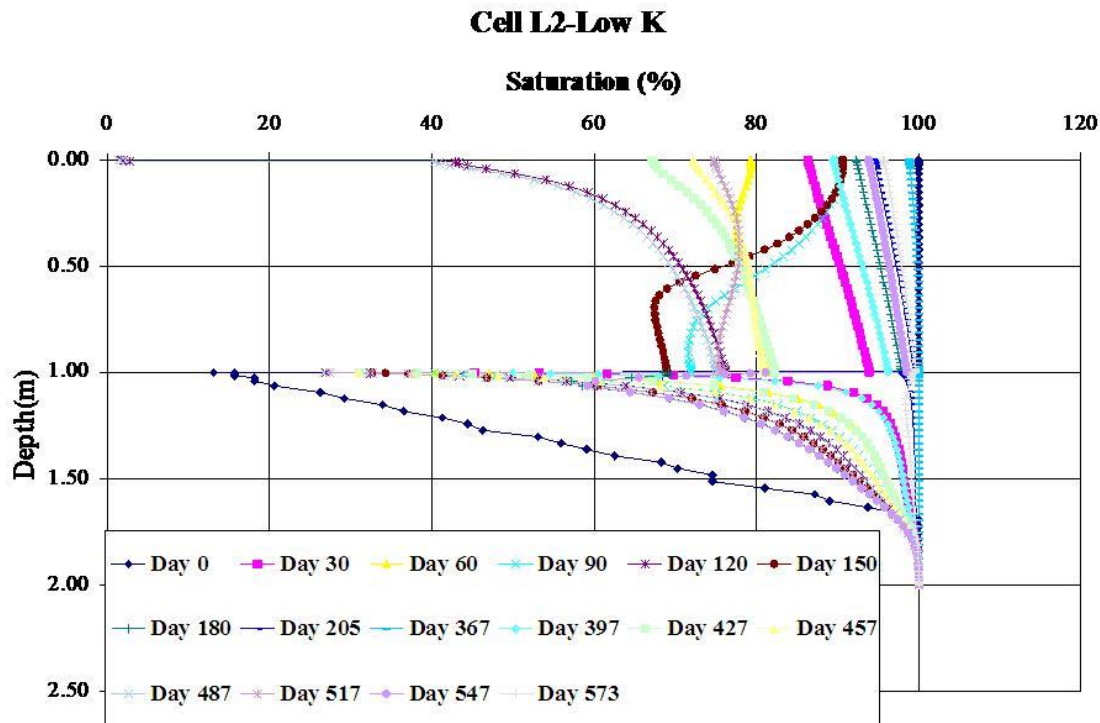
Figure 11. Saturation Profile for Cell L2.
