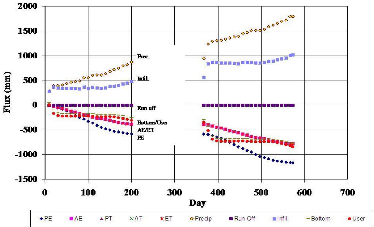
Figure 8. Flux summary for uncovered tailings.
