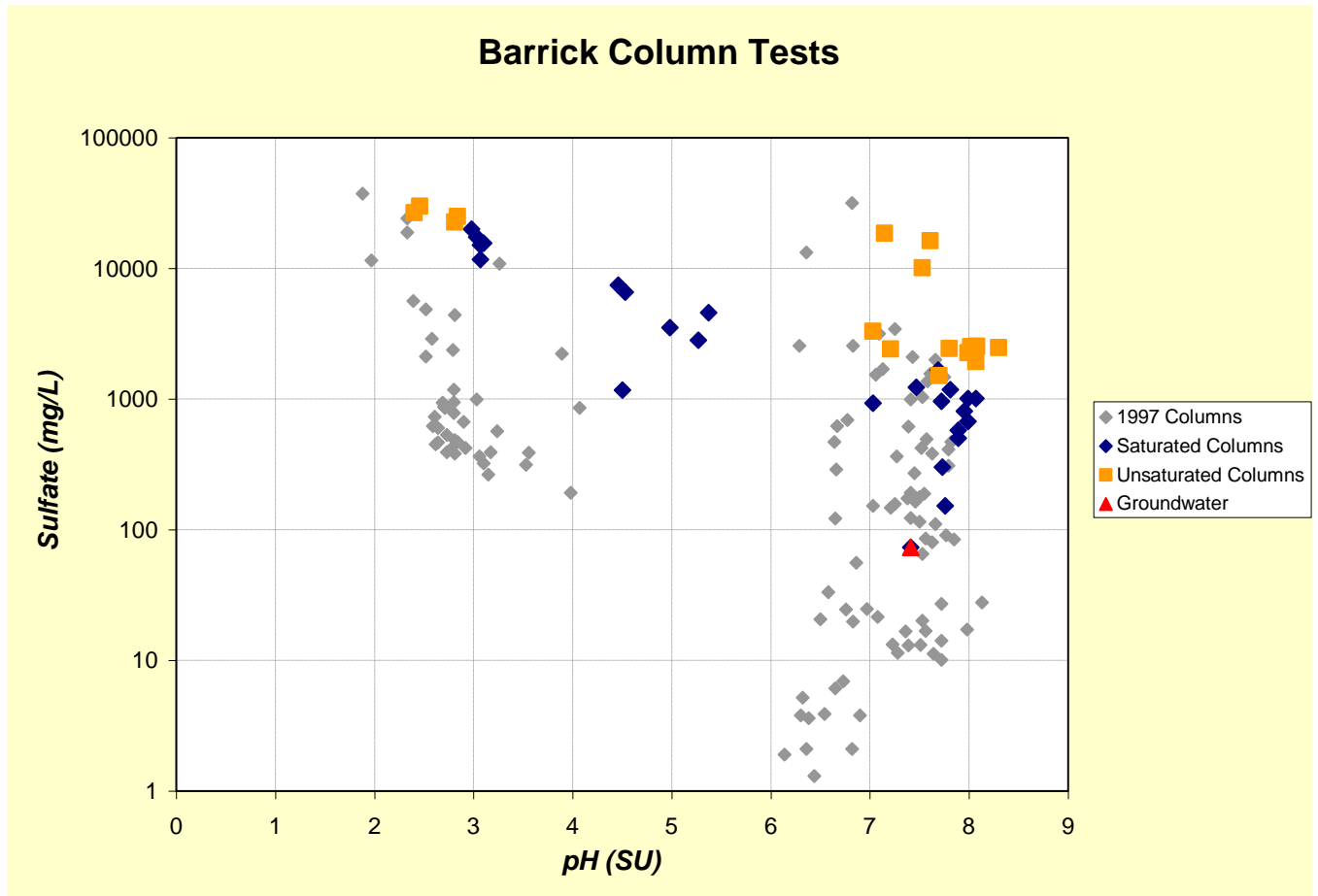
Figure 9. Relationship of solution pH and \text{SO}_4^{-2} for all samples collected from columns in 1997 and 2002.
