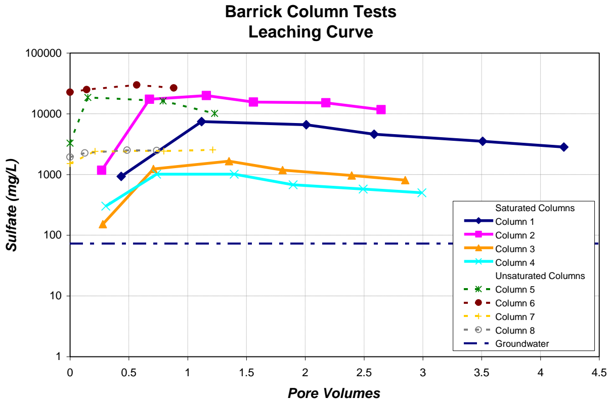
Figure 8. Changes in \text{SO}_4^{-2} concentration as a function of pore volumes displaced in the saturated and unsaturated columns
