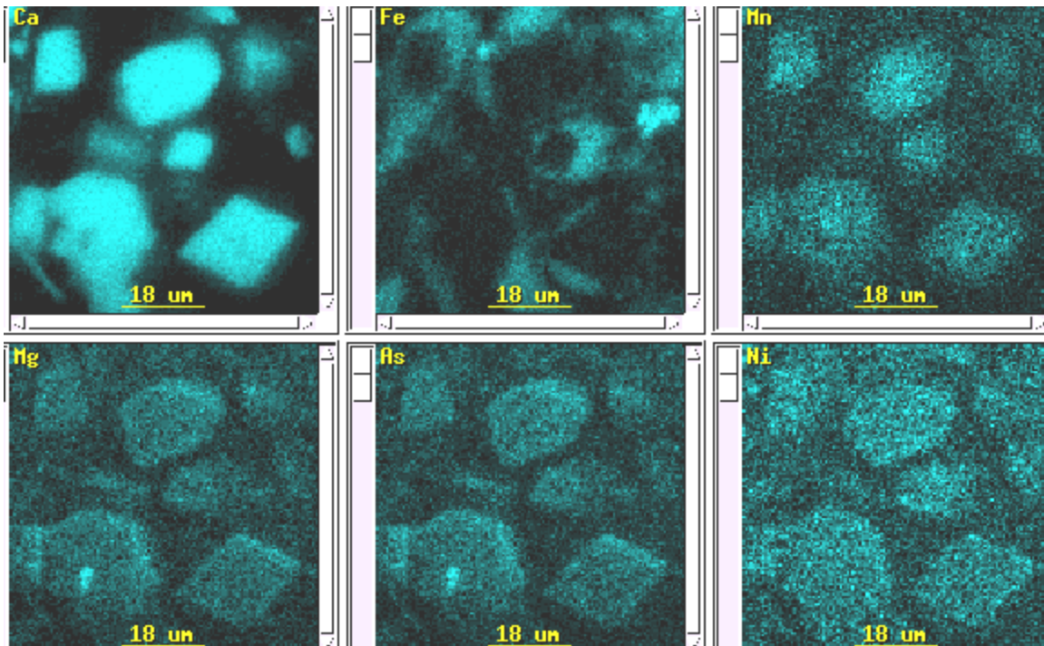
Figure 10. Carbonate grains in sample (02-485-B, evaporated 400 year pumped untreated). Arsenic and Mg showed slight enrichment towards the exterior of the grains, while core regions contained elevated levels of manganese. Iron was not present in any of the carbonate material.
