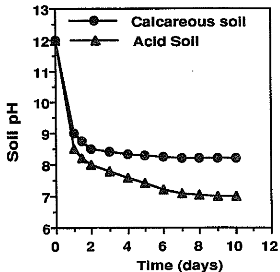
Figure 2. Change in soil pH with N-Viro Soil.
