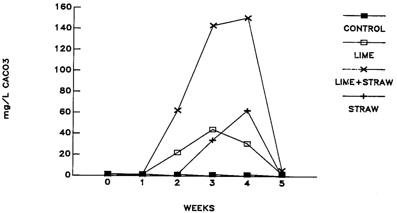
Figure 4: Alkalinity at the 3 m level in the experimental enclosures
