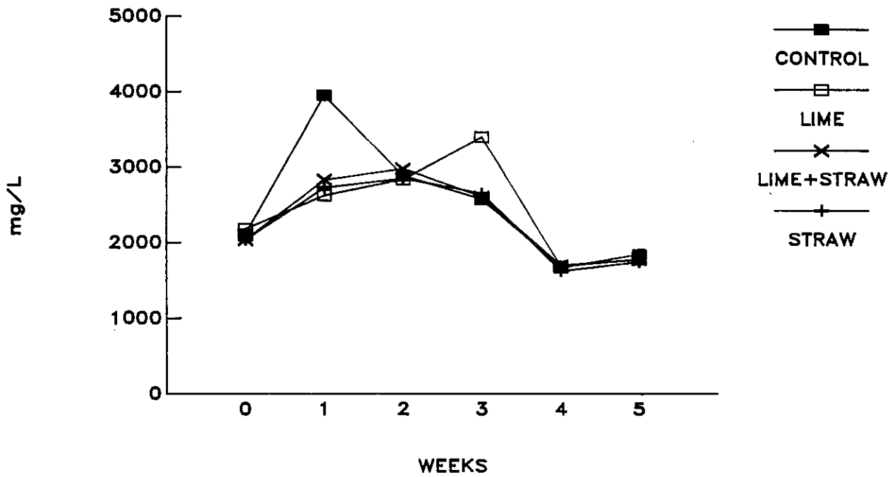
Figure 7: Sulfate concentrations at the 3 m level in the experimental enclosures.
