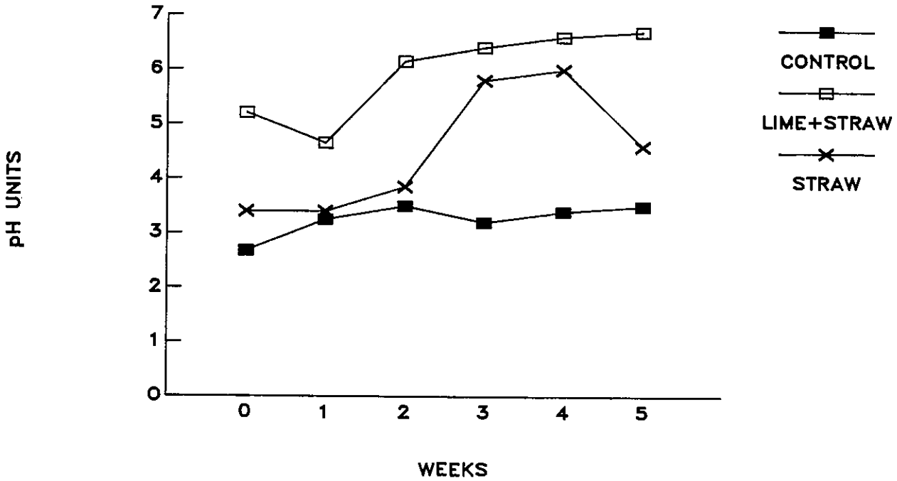
Figure 3: pH at the 3 m level in the experimental enclosures.
