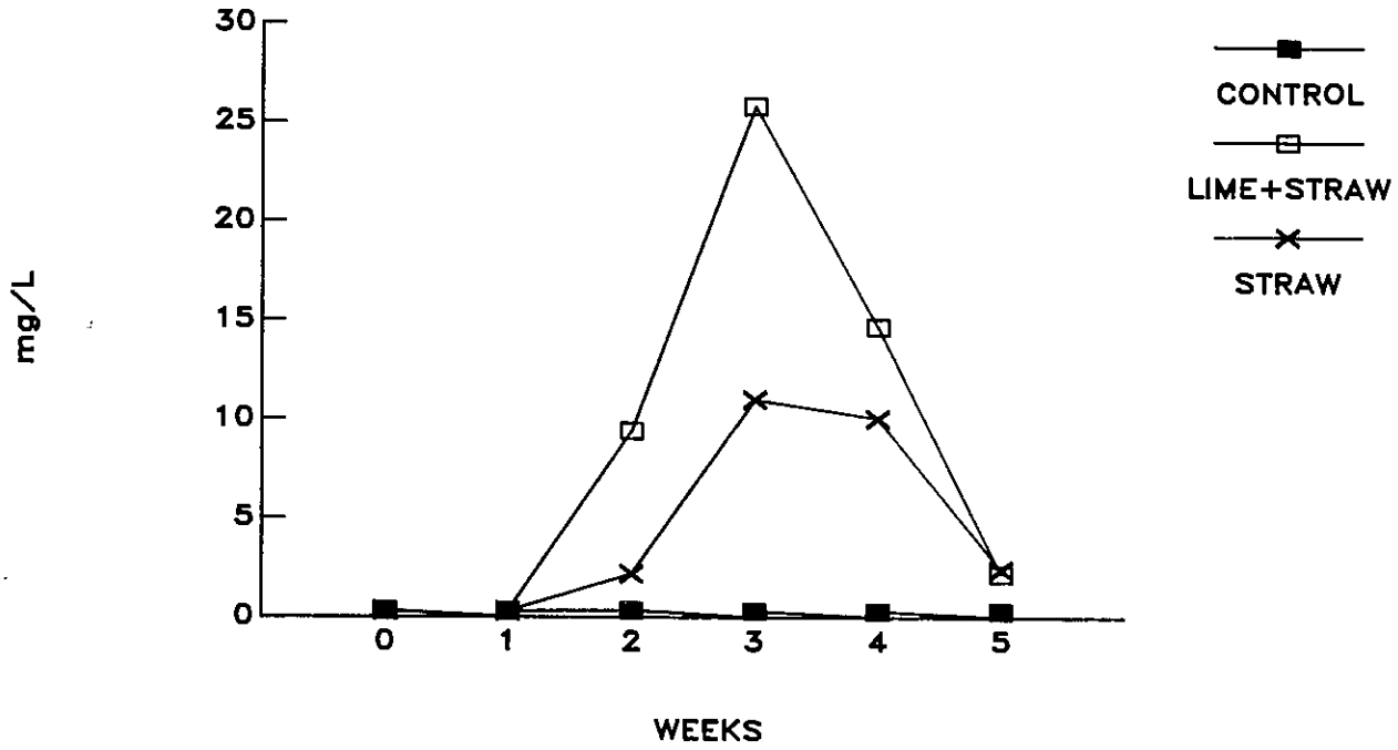
Figure 2.: Sulfide concentrations at the 3 m level in the experimental enclosures
